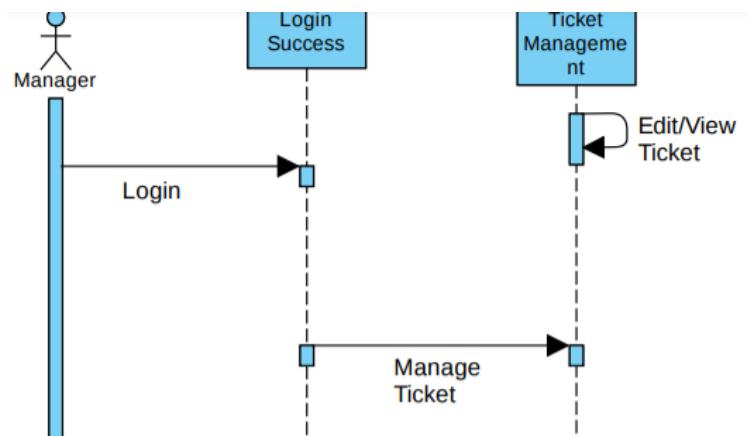
Fig 2.5.4.b Sequence Diagram for manager
