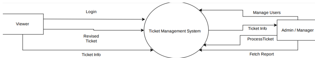
Fig 2.5.7.1 Data Flow Diagram 0 th level
