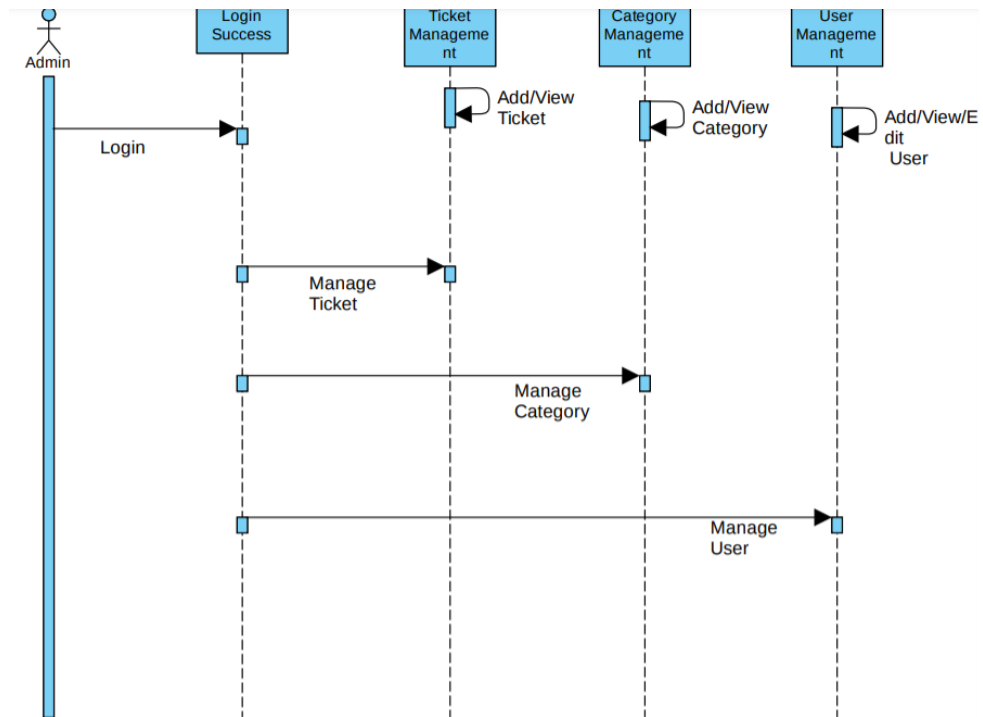
Fig 2.5.4.a Sequence Diagram for admin
