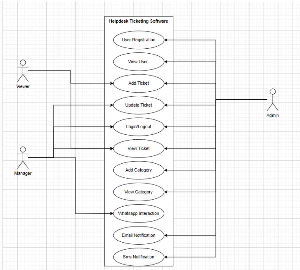
Fig 2.5.6 Use Case Diagram
