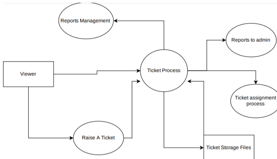
Fig 2.5.7.2 Data Flow Diagram 1 th level
