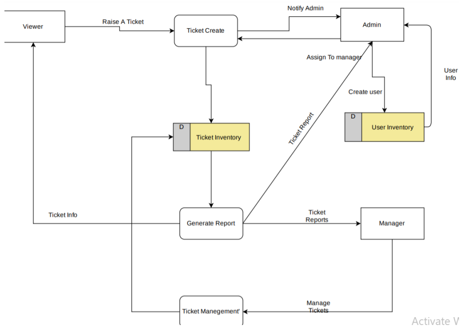
Fig 2.5.7.3 Data Flow Diagram 3 th level
