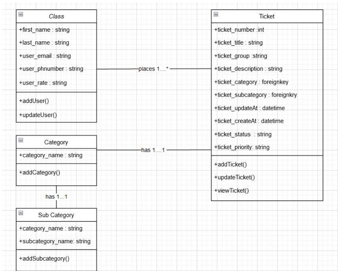
Fig 2.5.5 Class Diagram
