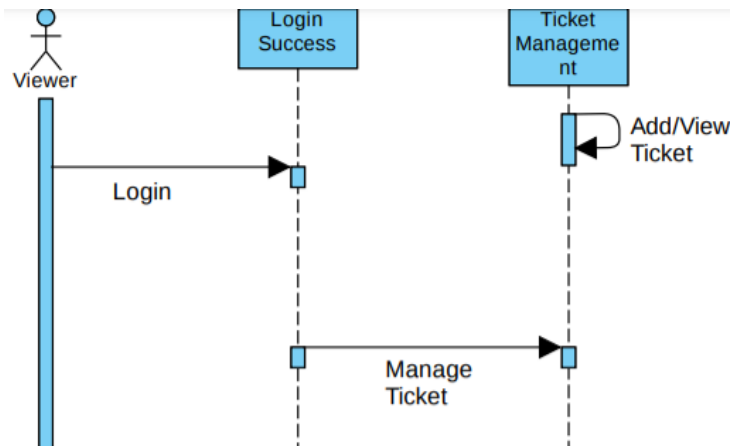
Fig 2.5.4.3 Sequence Diagram for viewer
