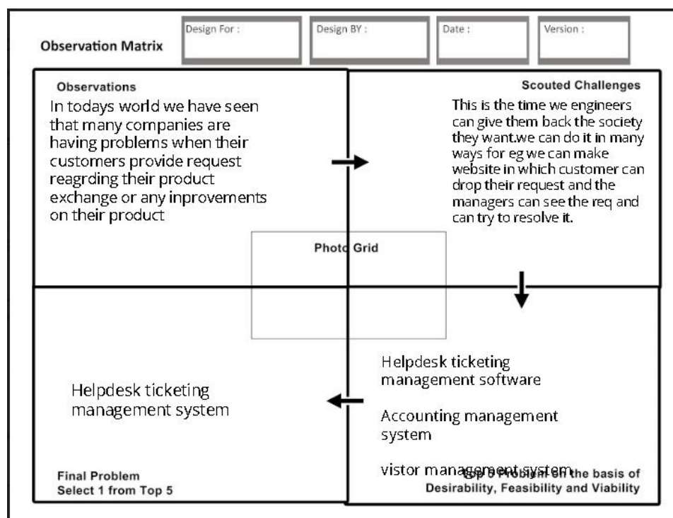
Fig 2.2.1 Observation Matrix
